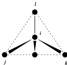
Fig. 5.24: Principle of improper dihedral angles. Out of tetrahedral angle. The improper dihedral angle \xi is defined as the angle between planes (i,j,k) and (j,k,l).
